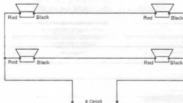
Figure 3 - Connection of four SRO/12 speakers in series-parallel
