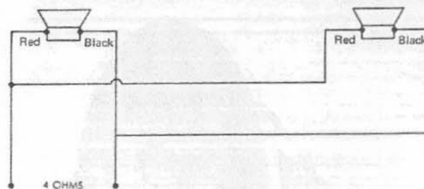
Figure 2 - Connection of two SRO/12 speakers in parallel
